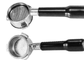
San Marco 3-Ear Bottomless Portafilter Material:Stainless Steel Size:54mm
